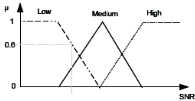
Figure 8: Membership functions of SNR
