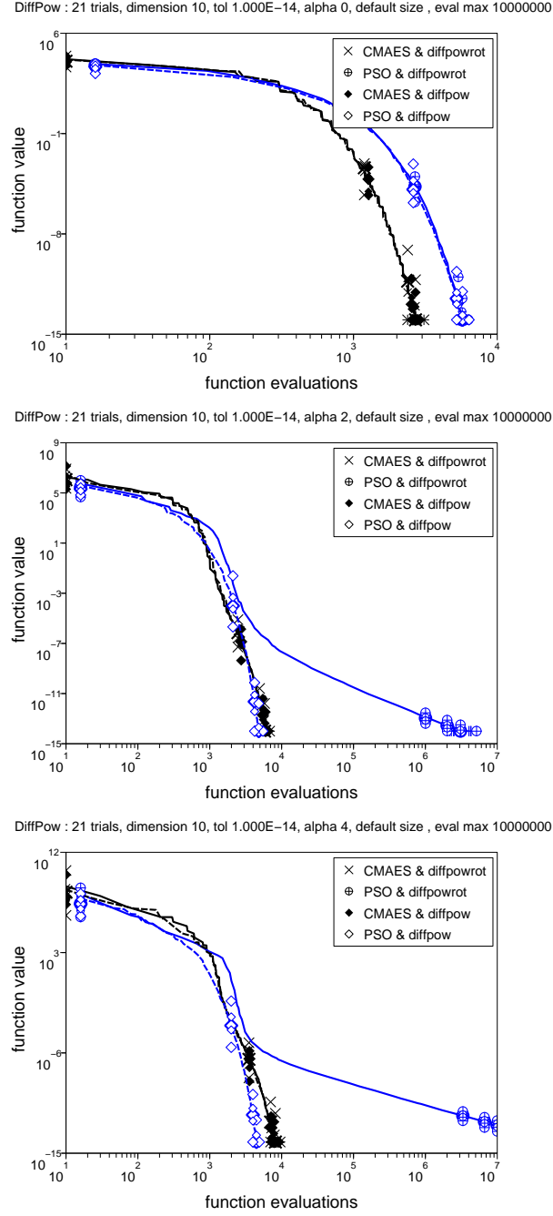
Figure 7: Diff-Powers function in 10-D: time evolution of the median function value, rotated and non-rotated case, with parameter \alpha = 0, 2, 4 , from top to bottom. Small symbols indicate the 25%- and 75%-ile, large symbols indicate smallest and largest value from 21 trials. S-PSO: \oplus, \diamond ; CMA-ES: \times, \blacklozenge
