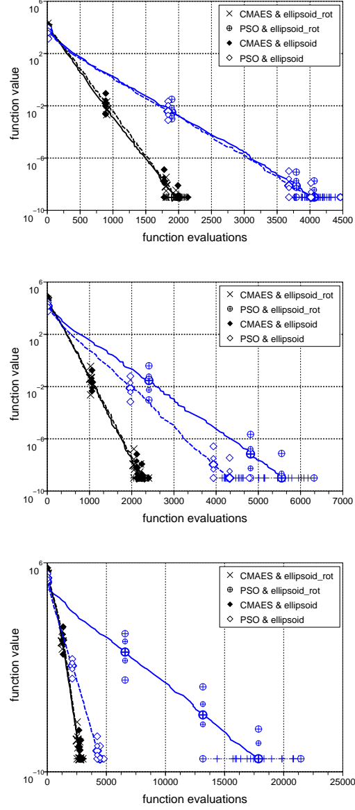
Figure 2: Ellipsoid function in 10-D: time evolution of the median function value with a function condition number \alpha of 1, 10, and 100, from top to bottom. Small symbols indicate the 25% and 75%-ile, large symbols indicate smallest and largest value from 21 trials. Solid lines: rotated function, dashed lines: non-rotated (separable) function. S-PSO: \oplus, \diamond ; CMA-ES: \times, \blacklozenge
