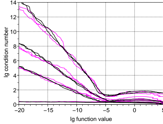
Figure 9: Diff-Powers function: log-log plot (base 10) of the condition number of the covariance matrix in CMA-ES versus the best function value per generation where \alpha = 0, 1, 2, 10 (bottom to top), in 10- and 30-D, two runs in each case. For large \alpha the larger dimension yields slightly larger final condition numbers. The target function value, 10^{-14} corresponds to a condition number of somewhat above 10^5 for \alpha = 2 , and somewhat below 10^{10} for \alpha = 10 .
