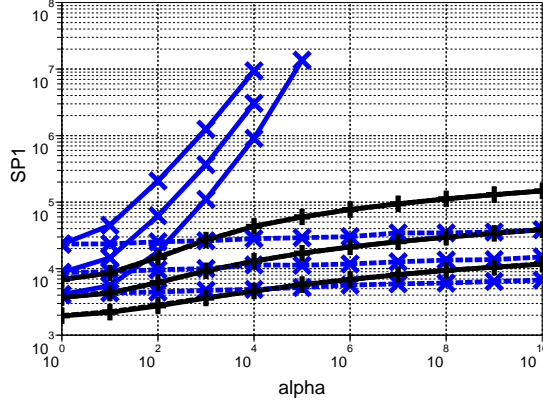
Figure 3: Ellipsoid function: \widehat{SP1} to reach f_{\text{target}} = 10^{-9} on the rotated (solid) and the non-rotated (dashed) function in dimensions 10, 20, 40 versus condition number \alpha . S-PSO: \times , CMA-ES: + . Up to the condition number of 10^3 the success rates are 100%. For condition numbers larger than 10^4 S-PSO regularly exceeds the maximum number of function evaluations of 10^7 .
