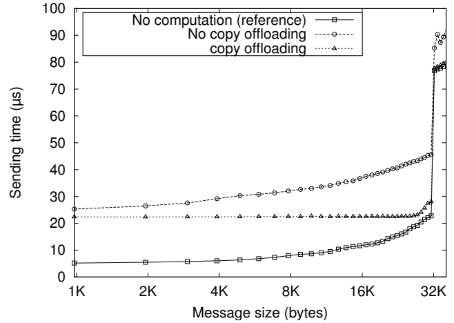
Figure 5. Small messages offloading results.
