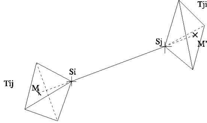
Figure 7: Edge-upwind tetrahedra
