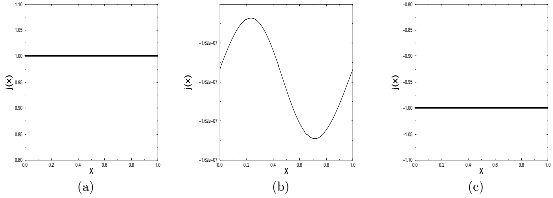
Figure 1: Macroscopic current as a function of the space variable for (a) t = 0 , (b) t = \pi/2 , (c) t = \pi .
