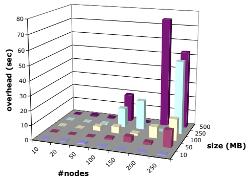
Figure 3: Evaluation of the BitDew overhead when transferring files.
