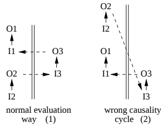
Figure 2: Causality cycle generation: O1, O2 and O3 signals are independent. But, when choosing a total order, we can introduce a causality cycle. If ordering (1) is chosen, in module final, taking into account the renaming, we obtain the system: \{ L1 = I, L2 = L1, O = L2 \} which is well sorted. At the opposite, if we choose ordering (2), in module final we get: \{ L2 = L1, O = L2, L1 = I \} which has a causality cycle.
