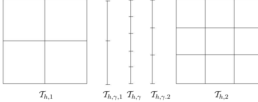
Figure 13: An example of a numerical discretization with nonconforming grids for the fracture and the subdomains
