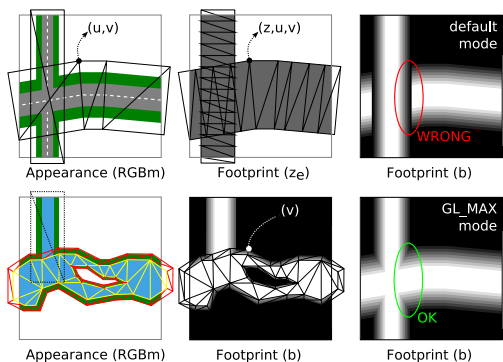
Figure 6: Appearance and footprint texture generation. Left: curves are drawn using a single strip. Areas are drawn using an interior mesh (yellow) and a border strip (red). Middle: Footprint generation. Right: b coefficients are combined in GL_MAX mode to ensure continuity.
