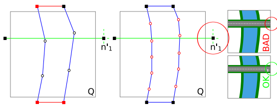
Figure 4: Clipping and refinement. Left: clipping of Q , the topleft subquad of P (Fig. 3). Curves are clipped conservatively. New curves are added, in red, to close clipped areas. Middle: refinement. Right: the stop line before the (clipped) crossing is missed with n_1 's topology (1 adjacent curve). Using instead n_1 's topology (4 adjacent curves) fixes this.
