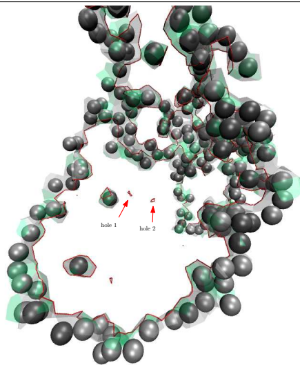
Figure 10 Boundary of the AB interface of complex 1A59 (red line), interfacial water (gray spheres), and AW - BW interface (grey and green Voronoi polygons). The holes pointed out by arrows prevent the shelling order from peaking in the middle of the interface patch –compare to the bottom left panel of complex 1A59 on Fig. 8.
