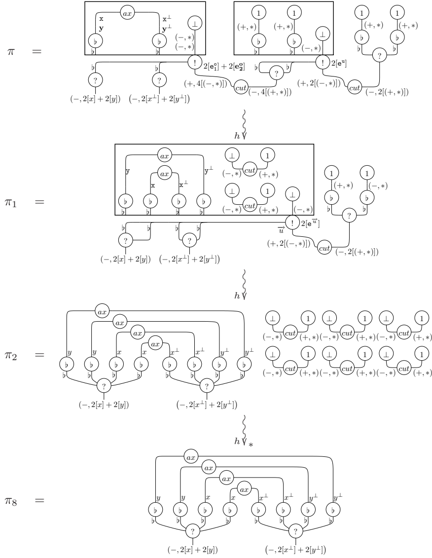
Figure 10: example of an experiment e : \pi and its residues under cut reduction. The value of an experiment on an edge or ! -link is written as a label of that edge/ ! -link. Inside the box we use different styles to describe different experiments: in particular in the left box (resp. right box) of \pi , we write in typewriter the values of e_1^o (resp. e^u ) and in bold the values of e_2^o . For simplicity we have omitted the values on the structural edges.
