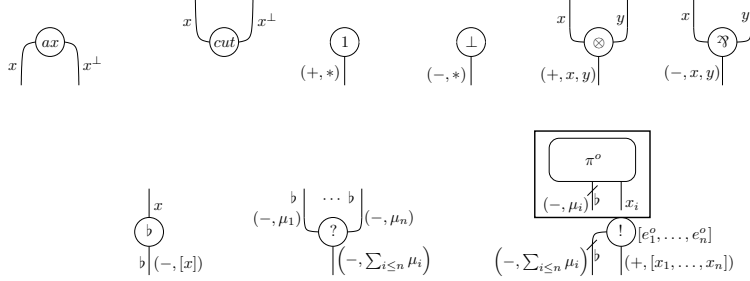
Figure 9: experiments of pure proof-structures
