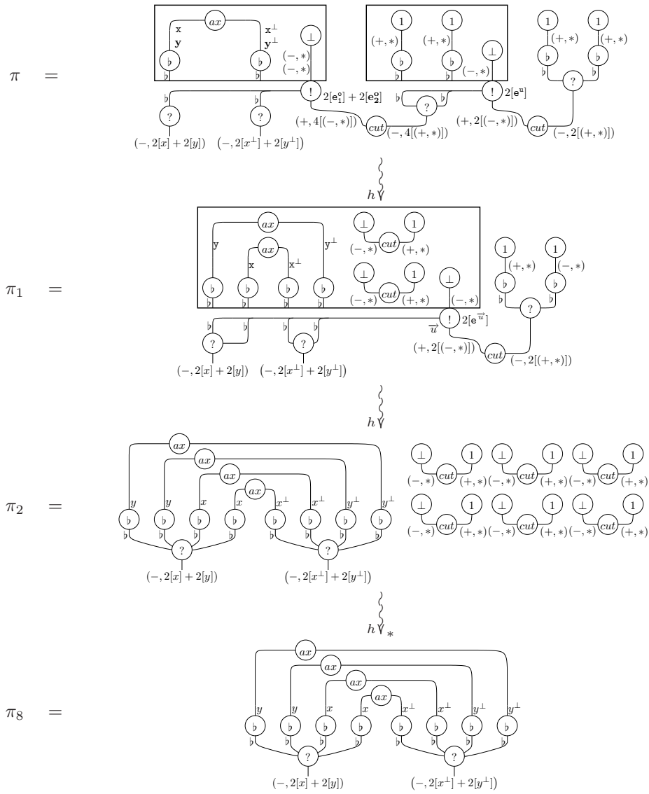
Figure 10: example of an experiment e : \pi and its residues under cut reduction. The value of an experiment on an edge or !-link is written as a label of that edge/!-link. Inside the box we use different styles to describe different experiments: in particular in the left box (resp. right box) of \pi , we write in typewriter the values of e_1^o (resp. e^a ) and in bold the values of e_2^o . For simplicity we have omitted the values on the structural edges.
