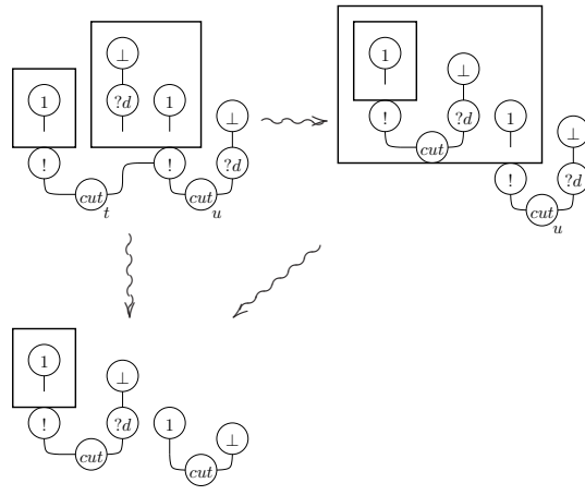
Figure 8: example of two head reductions with different length in the “traditional syntax”: reducing first the cut t and then the cut u gives the same result as reducing at once u . The reader can check that in our syntax both t(\pi) and u(\pi) reduce in exactly one step to the same net.
