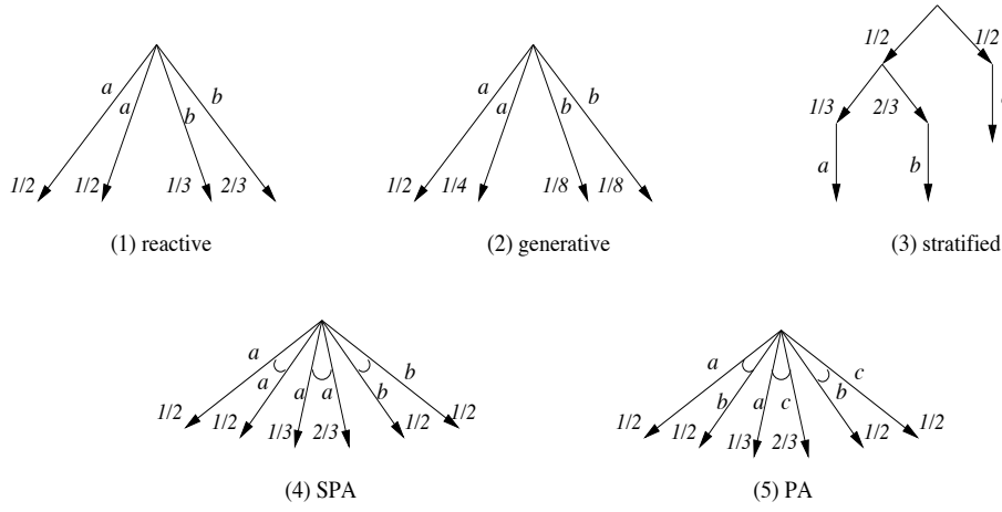
Fig. 1. Probabilistic models
