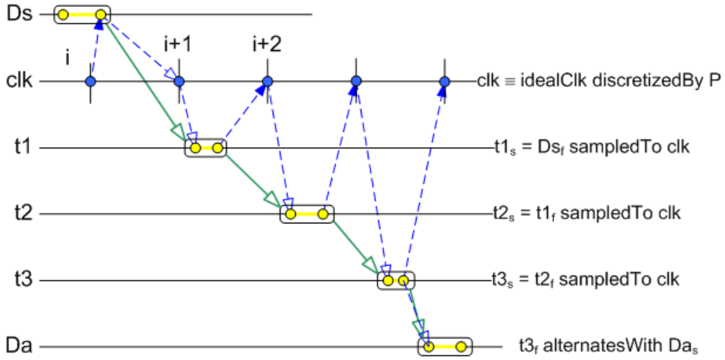
Figure 12. CCSL constraints, the synchronous case.
