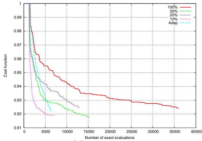
(b) Seed = 319
