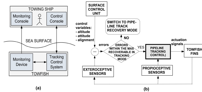
Fig. 6. Control system schemes
