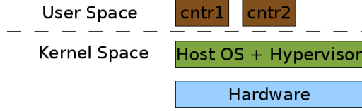
Figure 3: Container Based Virtualization
