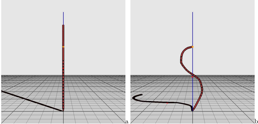
Figure 3: Chain example. This chain is composed of 30 segments with 3 rotational degrees of freedom each (a) Initial configuration (b) final configuration.
