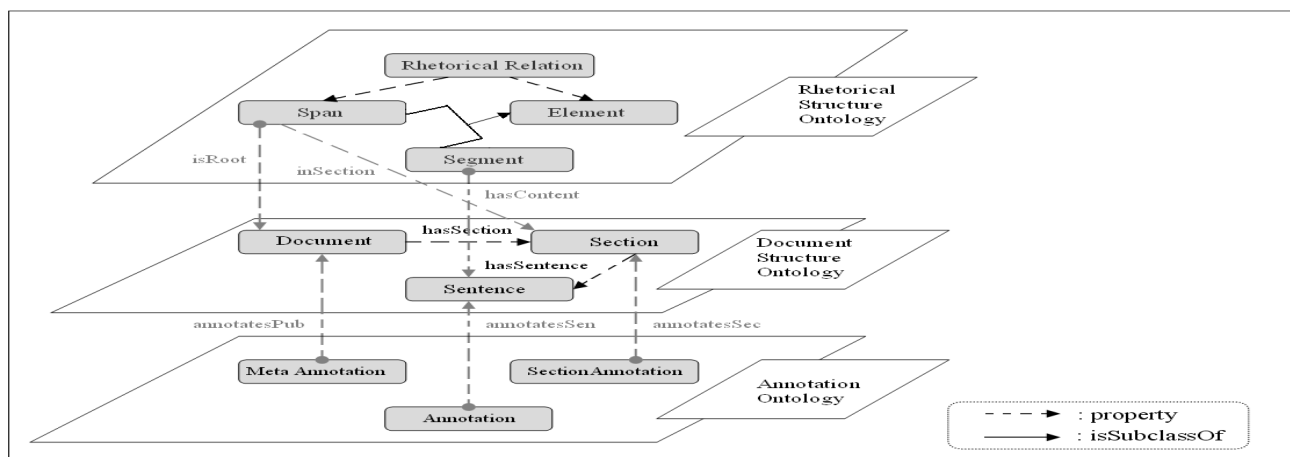
Figure 2: Ontology Layers
