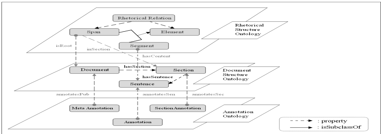
Figure 2: Ontology Layers
