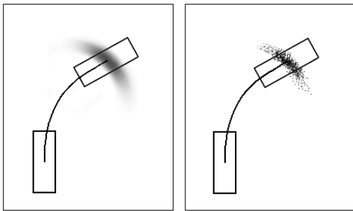
Fig. 4. The probabilistic velocity motion model P(x_t | x_{t-1}, u_t) of the vehicle (left) and its sampling version (right).
