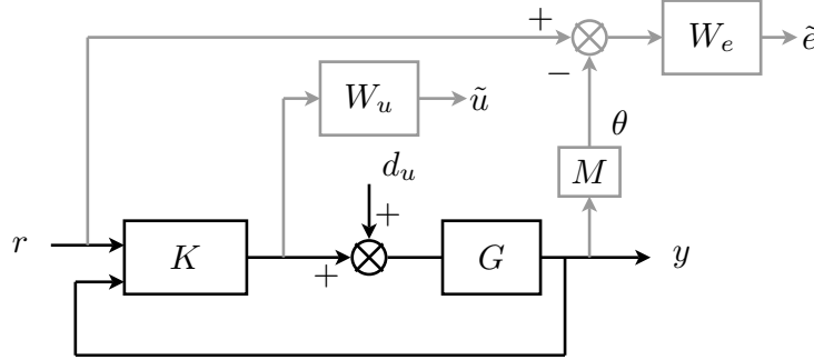
Figure 8: General control configuration
