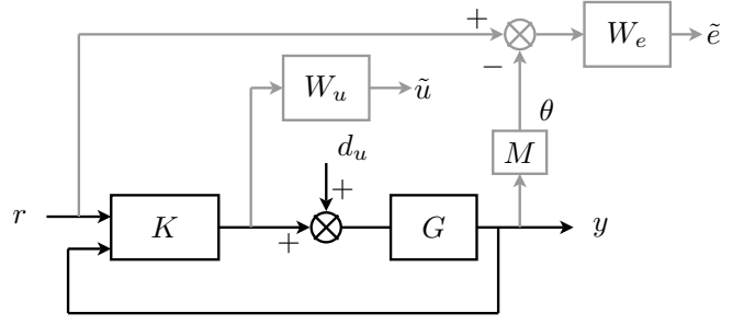
Fig. 7. General control configuration
