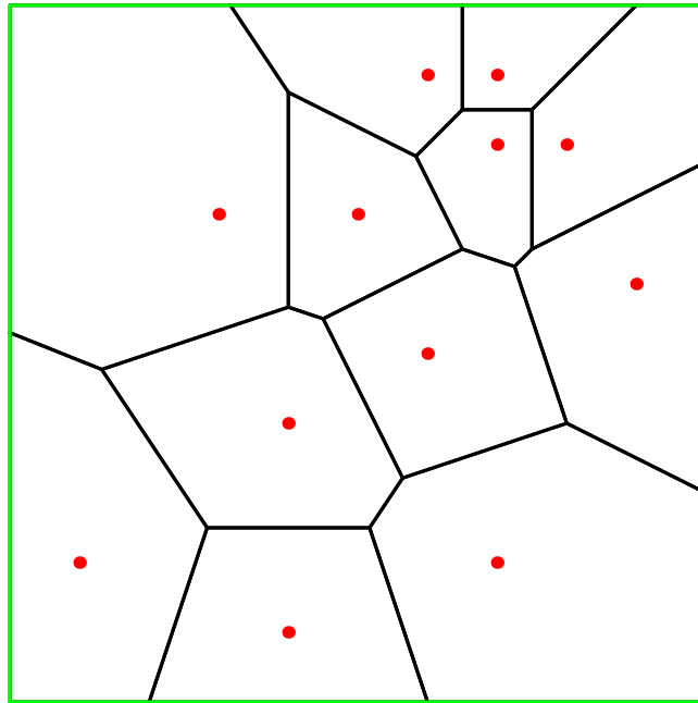
Figure 8.2: A Voronoi diagram
