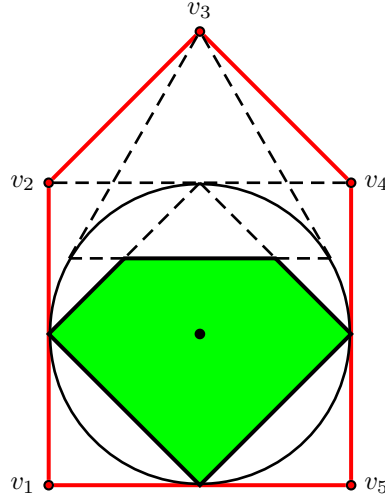
Figure 3.7: The polar dual of a polygon
