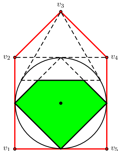
Figure 3.7: The polar dual of a polygon
