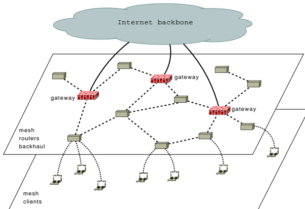
Figure 1: Example of a WMN topology
