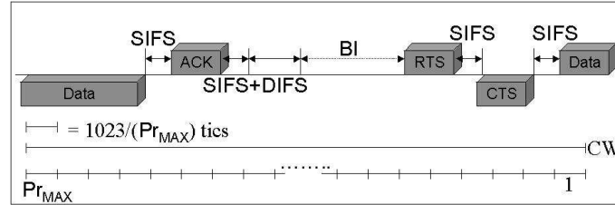
Figure 6: The contention mechanism in DB-MAC [16]
