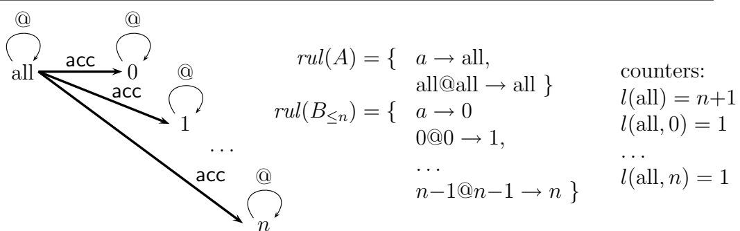
Figure 6: Rule (frb 2 ) can infer, for all 0 \leq i \neq j \leq n , the clause \text{frb}(\text{all}, i) :- \text{acc}(\text{all}, j) .
