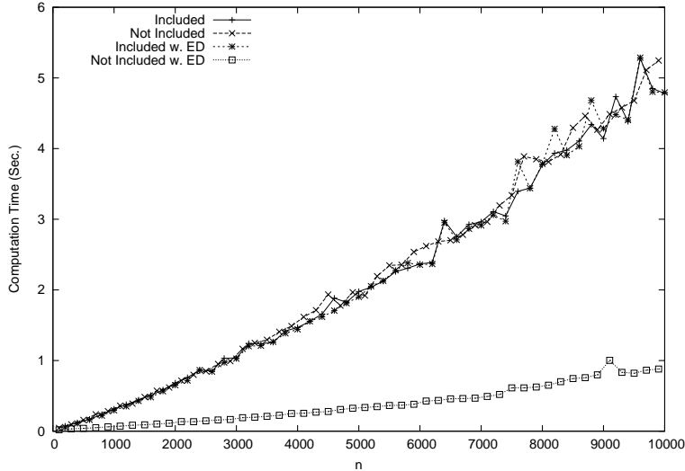
Figure 23. Average computation time for testing L(Mult2_n) \subseteq L(Mult2_{200}) .
