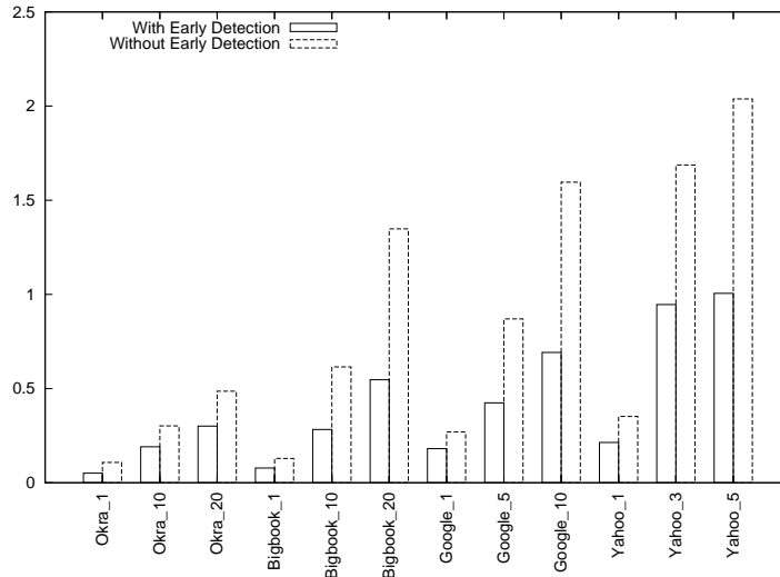
Figure 24. Average computation time (in Sec.) of learning sessions with and without early detection of failure fail_1 .
