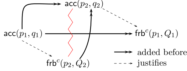
Figure 11. Early failure detection: \text{frb}^c(p_2, q_2) in \text{lfp}(D_2(A, B)) before \text{acc}(p_2, q_2) .
