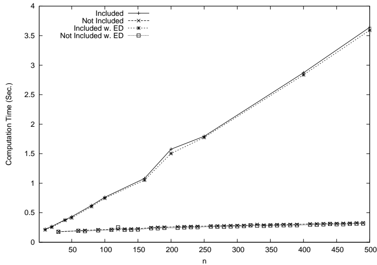
Figure 22. Computation time for testing L(Mult_{400}) \subseteq L(Mult_n) .
