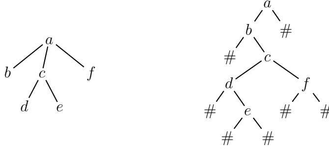
Figure 25. The tree a(b, c(d, e), f) and its firstchild-nextsibling encoding a(b(\#, c(d(\#, e(\#, \#))), f(\#, \#))), \#) .
