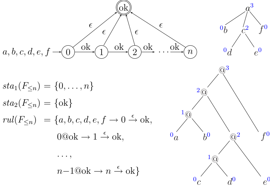
Figure 12. On the left, we define for all n a deterministic factorized tree automaton F_{\leq n} . On the right, the lower tree is the Curried encoding of the upper. We annotate all nodes by the unique state assigned by the evaluator of the deterministic tree automaton b(F_{\leq n}) where n \geq 3 .
