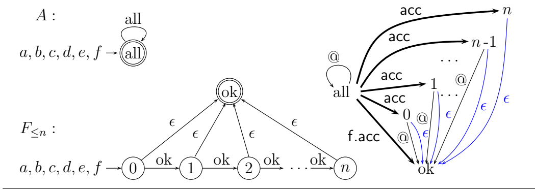
Figure 17. Example run of the algorithm: \text{f.frb}_1^c(\text{all}, \{0, \dots, n-1\}) is inferred.
