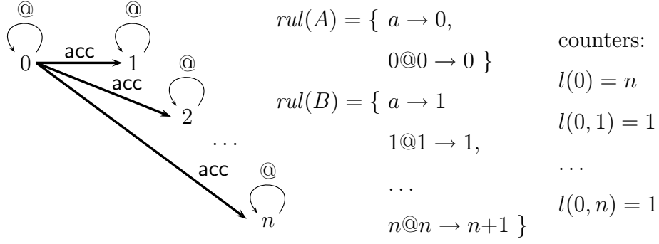
Figure 6. Rule (\text{frb}_{/2}) can infer, for all 1 \leq i \neq j \leq n , the clause \text{frb}(0, i) :- \text{acc}(0, j) .
