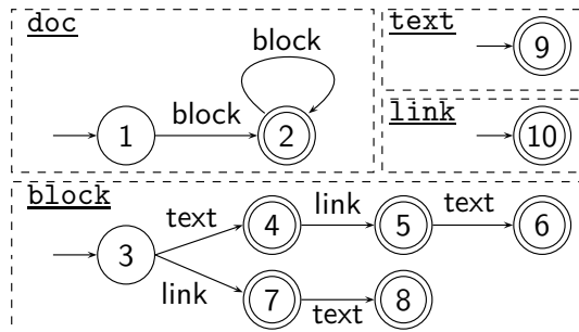
Figure 19. An example DTD and the corresponding Glushkov automata.
