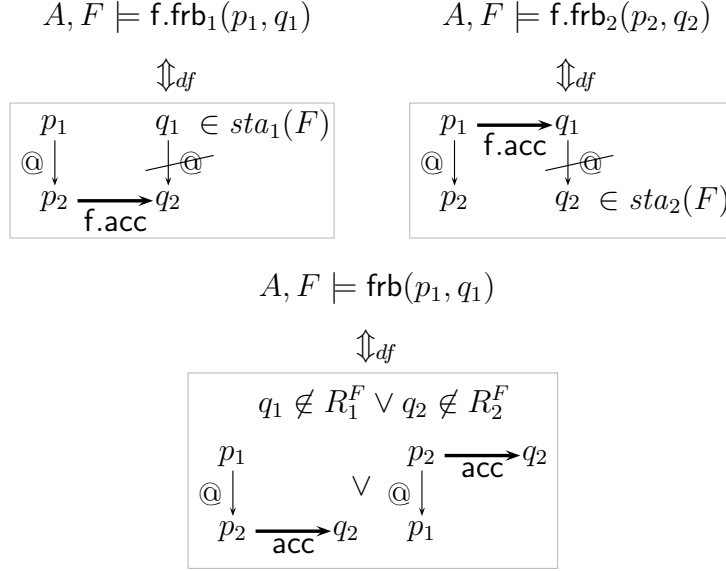
Figure 14. Semantics of predicates \text{f.frb}_1 , \text{f.frb}_2 and \text{frb} for factorized tree automata.
