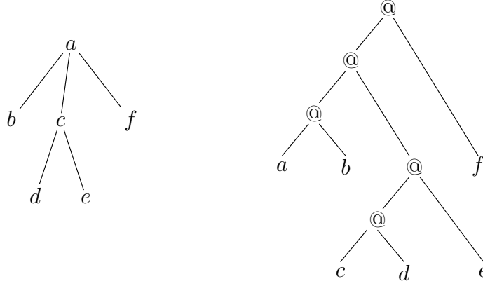
Figure 1. Currying the ranked tree a(b, c(d, e), f) into the binary tree a@b@(c@d@e)@f .
