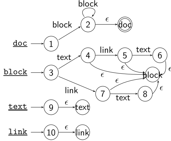
Figure 20. A representation of the deterministic factorized tree automaton for the DTD in Figure 19. Alphabet \Sigma is \{\text{doc}, \text{block}, \text{text}, \text{link}\} , states of sort 1 are \{1, \dots, 10\} and states of sort 2 are \{\text{doc}, \text{block}, \text{text}, \text{link}\} . A constant rule is for instance \text{doc} \rightarrow 1 , a binary rule 2@ \text{block} \rightarrow 2 and an \epsilon -rule 2 \xrightarrow{\epsilon} \text{doc} .
