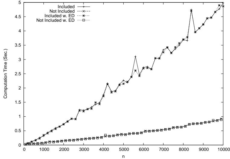
Figure 21. Computation time for testing L(Mult_n) \subseteq L(Mult_{200}) .
