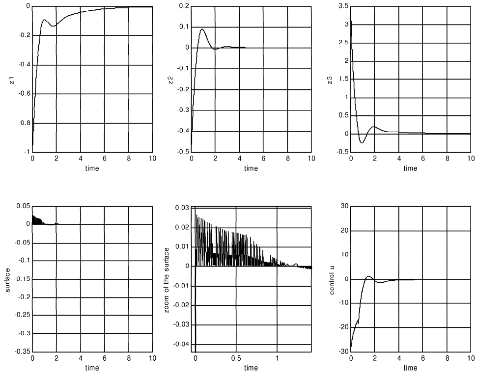
Figure 2: Response of the closed-loop system (22), (13) with \tau = 0.63 and \varepsilon = \frac{1}{2} .
