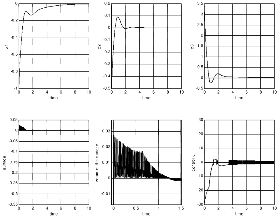
Figure 1: Response of the closed-loop system (22), (13) with \tau = 0.63 and \varepsilon = 0 .
