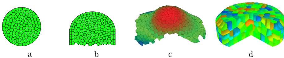
Figure 12: Tissue models.
