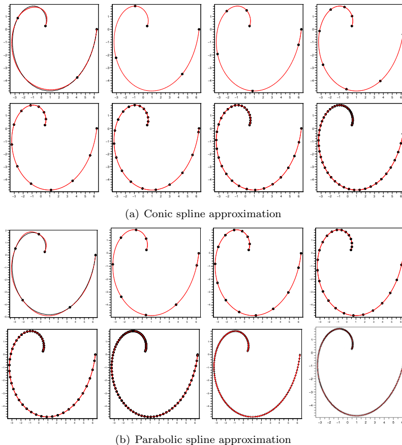
FIGURE 4. Approximation of the spiral for \varepsilon ranging between 10^{-1} to 10^{-8} .
