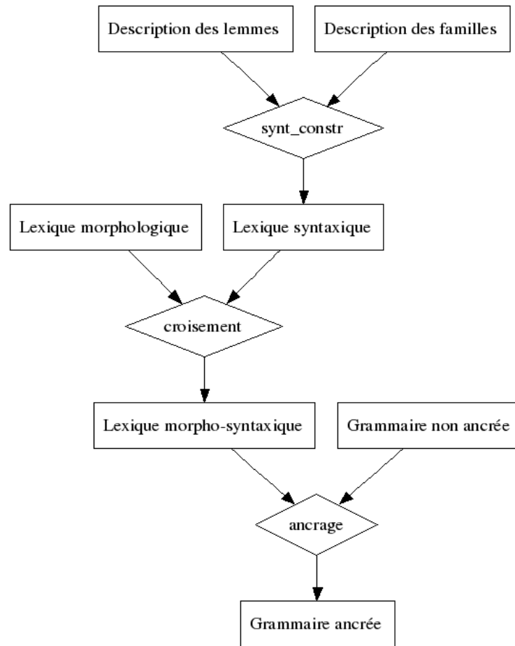
FIG. 3.2 – Architecture de LEOPAR.
