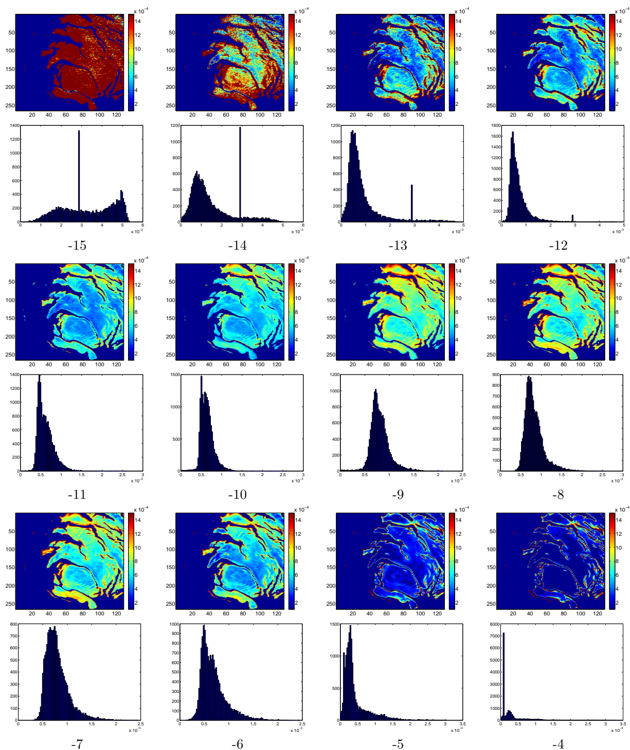
Figure E.0.1: Studied image: during orbit 41. Proportion of Water.
