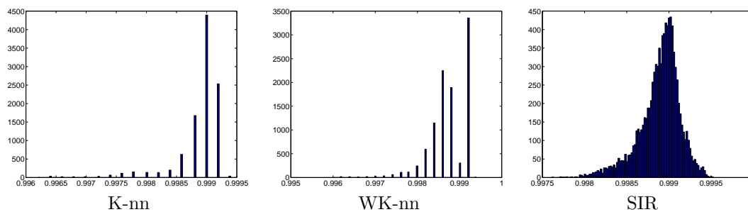
Figure 4.5.38: Studied image: during orbit 103. Histogram of the proportion of CO 2 .
