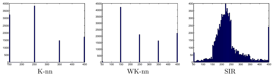
Figure 4.5.32: Studied image: during orbit 61. Histogram of the grain size of water.
