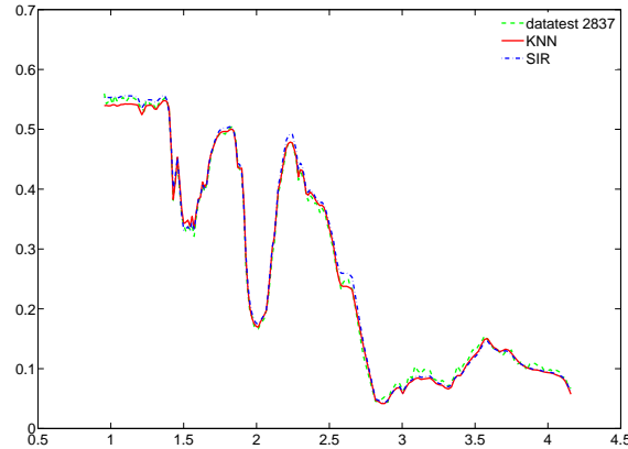
Figure 4.1.1: Analyzing the K-nn results for one spectrum of Tdata. Ldata 2. Horizontally: Wavelengths, Vertically: Reflectance.
