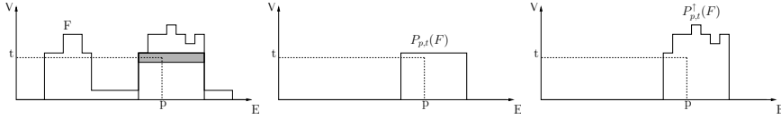
Figure 1. Decomposition of a function into its peak components. Left: Original function F . In grey: connected component of X_t(F) including p . Middle: Peak component P_{p,t}(F) . Right: Lobe component P_{p,t}^{\uparrow}(F) .
