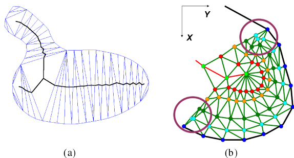
Figure 2: Limitations of the Teddy approach: (a) the skeleton extracted from the CDT (Constrained Delaunay Traingulation) has some discontinuities and, (b) the sampling of the internal edges leads to very tiny and uneven triangles.
