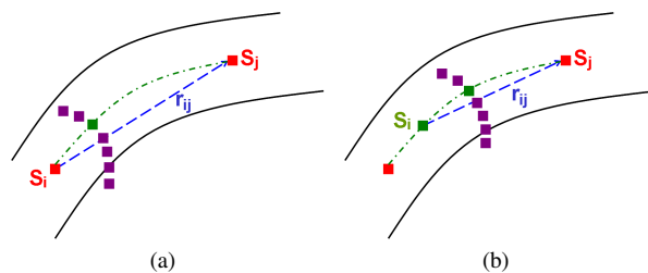
Figure 6: Creation of new skeleton points. The local minimum of the implicit function is the green dotted line; green points are the added skeleton points while violet points are the non-local minimums of the implicit function evaluation. (a) Starting from the first seed, a new skeleton point is added (corresponding to a local minimum). (b) The new point becomes the new starting point.
