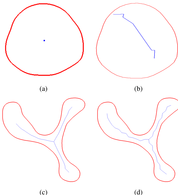
Figure 12: Comparison between the skeleton of Teddy (b)-(d) and ours (a)-(c). Thanks to implicit curve our algorithm manages to create a good skeleton (one point) for circular silhouette curves. Besides, for more complex silhouette curves, the skeleton extracted by our technique is smoother.
