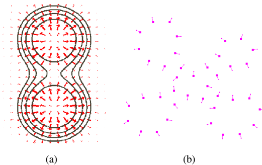
Figure 3: (a) Gradient field of an implicit surface (from [26]). (b) Silhouette points used to reconstruct the 2D variational implicit surface.
