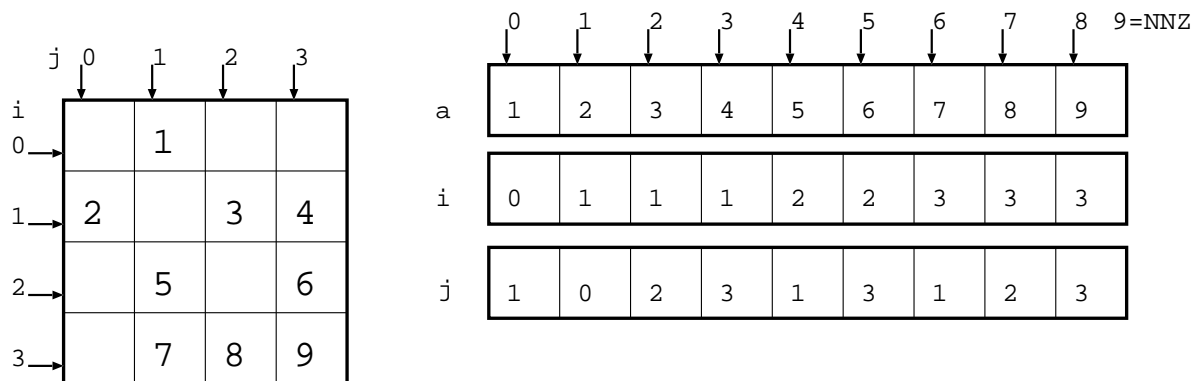
Figure 10.1: Example of sparse matrix with TRIAD format
