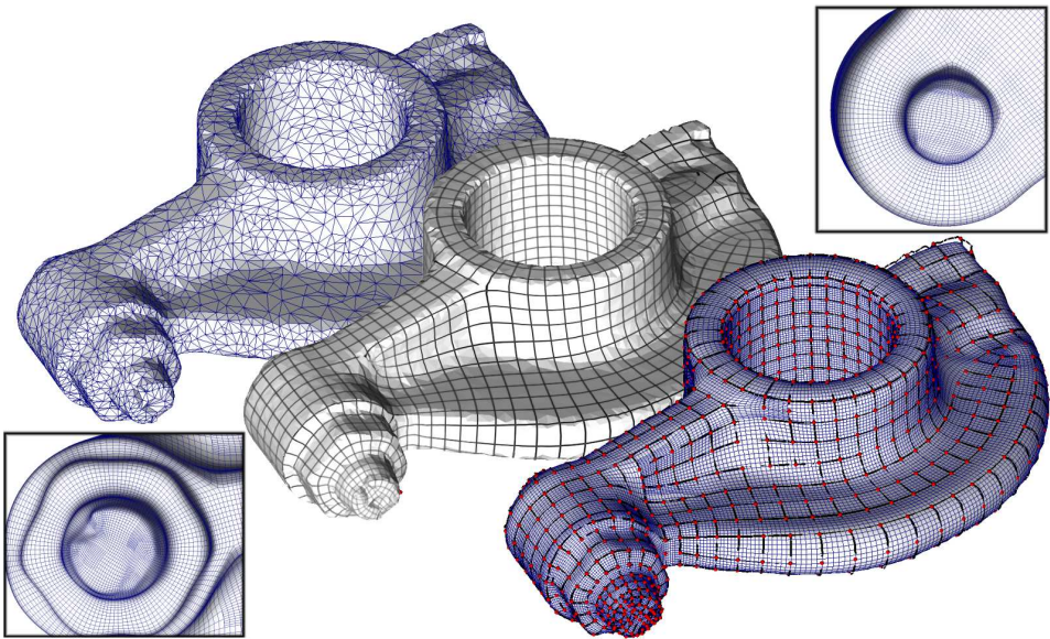
Figure 1.4: A global parameterization realizes an abstraction of the initial geometry. This abstraction can then be re-instanciated into alternative shape representations.
