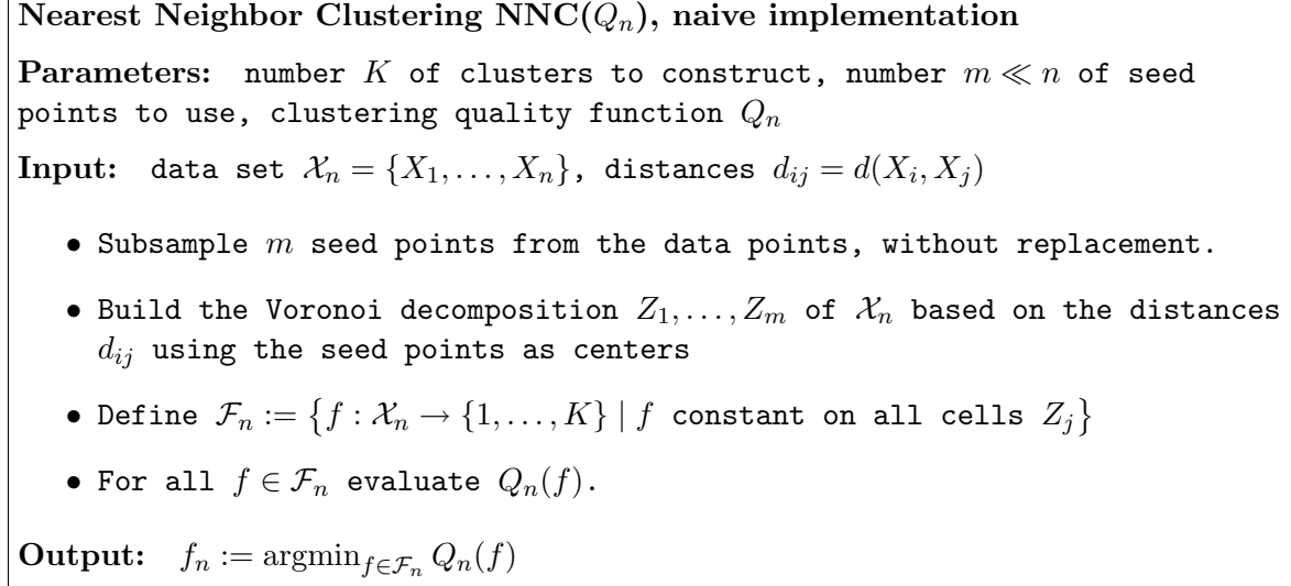
Figure 1: Nearest neighbor clustering for a general clustering objective function Q_n .
