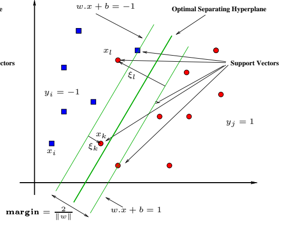
Figure 2: Soft margin case.
