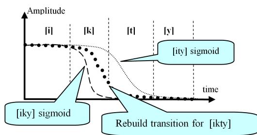
Figure 3: A V_1C...CV_2 reconstruction of the stretching profile of /ikty/ using consonant completion
