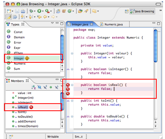
Figure 3. Interface at the second site after integration of ghost operations
