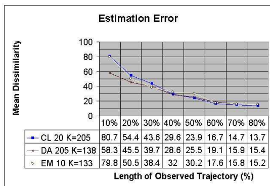
Fig. 4. Estimation errors for different techniques.
