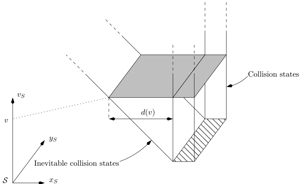
Figure 1: Collision states vs inevitable collision states.
