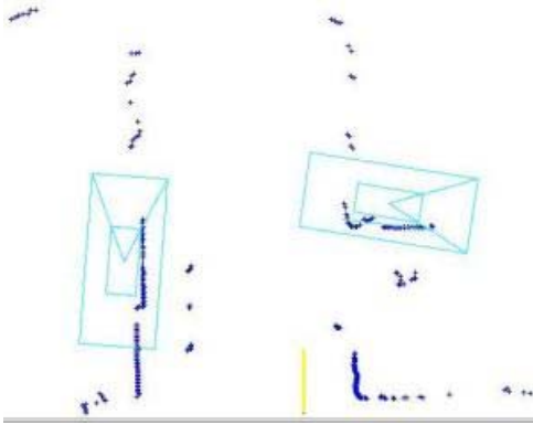
Fig. 8: The same configuration as in figure 7 but with rejected vehicle hypothesis in their inner and outer bounding boxes after stage 2 of vehicle detection
