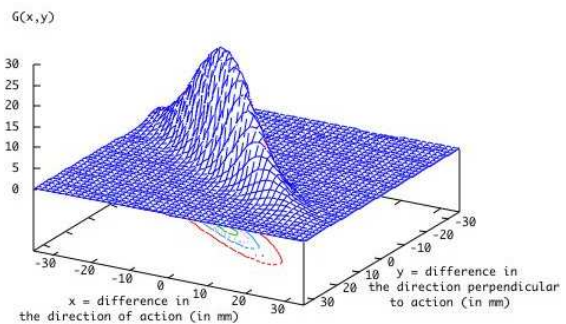
Fig. 5. Transition function of an arc-of-circle motion obtained after learning
