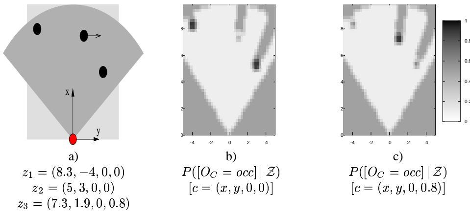
Fig. 3. Example of a grid estimation using a single laser sensor located at (0, 0) , in a scene including two stationary objects and an object moving from the left to the right at a velocity of 0.8 \text{ m/s} . In this example, the robot is not moving. The occupancy probability value of each cell is represented by a gray level (see the colors correspondences on the right side of the figure). (a) The sensed environment and the three instantaneous sensor observations expressed in the (x, y, \dot{x}, \dot{y}) space. (b) Occupancy probability in a 2-dimensional slice of the grid corresponding to a null relative velocity ( i.e. c = [x, y, 0, 0] ). (c) Occupancy probability in a 2-dimensional slice of the grid corresponding to a relative horizontal velocity 0.8 ( i.e. c = [x, y, 0, 0.8] ).
