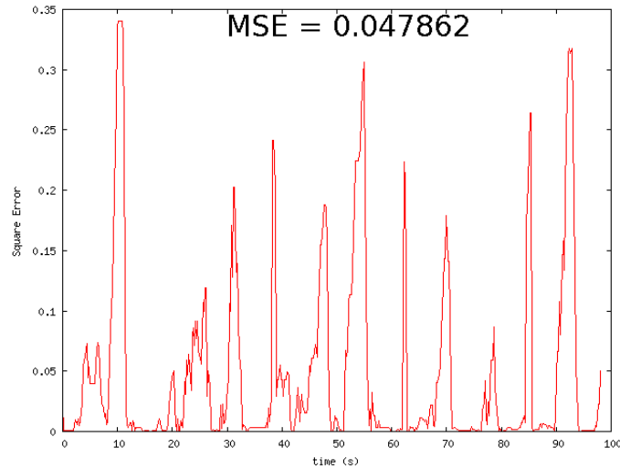
Figure 5.4: Square Error between human and auto driving
