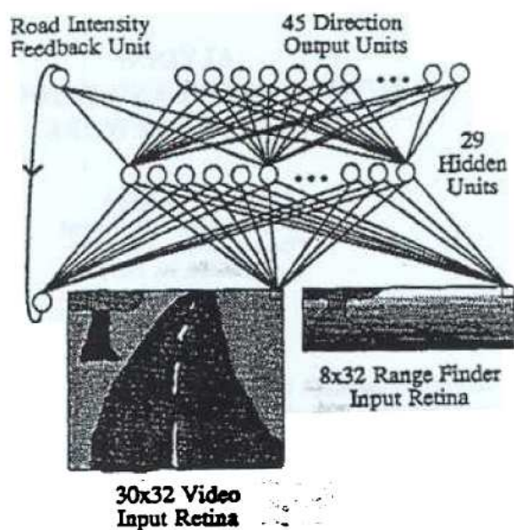
Figure 2.1: The ALVINN architecture [6]
