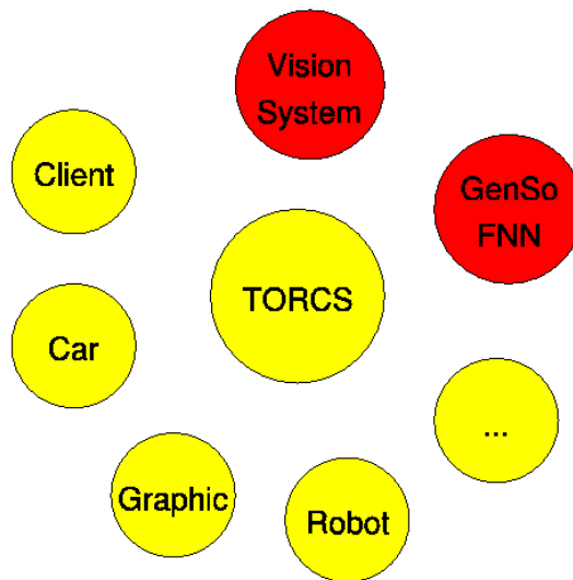
Figure 3.3: TORCS Modules
