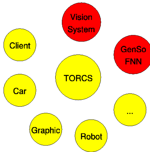
Figure 3.3: TORCS Modules
