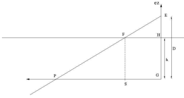
Fig. 11. Calculus of the position S of front vertices of the occupied area. They lie on the lines that join the orthogonal projection G of the camera on the ground and the homography projection P of the bottom of the bounding box on the ground. The distance GS is obtained thanks to the Thales theorem (Eq. 7).
