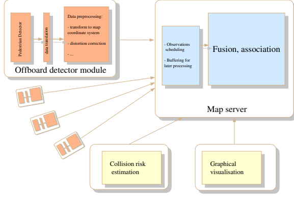
Fig. 3. The ParkView platform software organization
