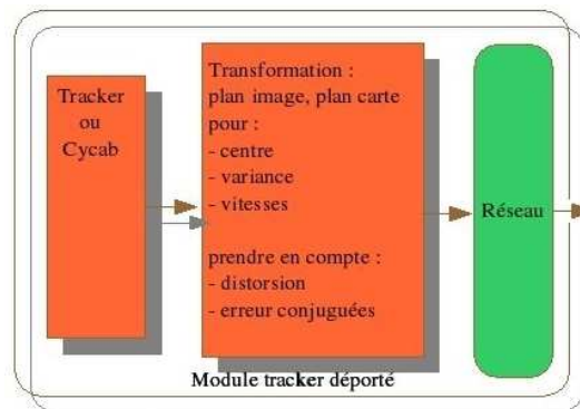
FIG. 8.22 – Le trackerConnector
