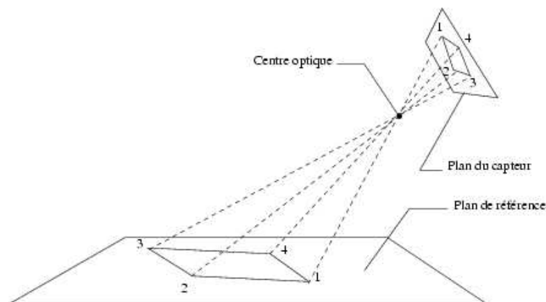
FIG. 6.1 – Projection centrale
